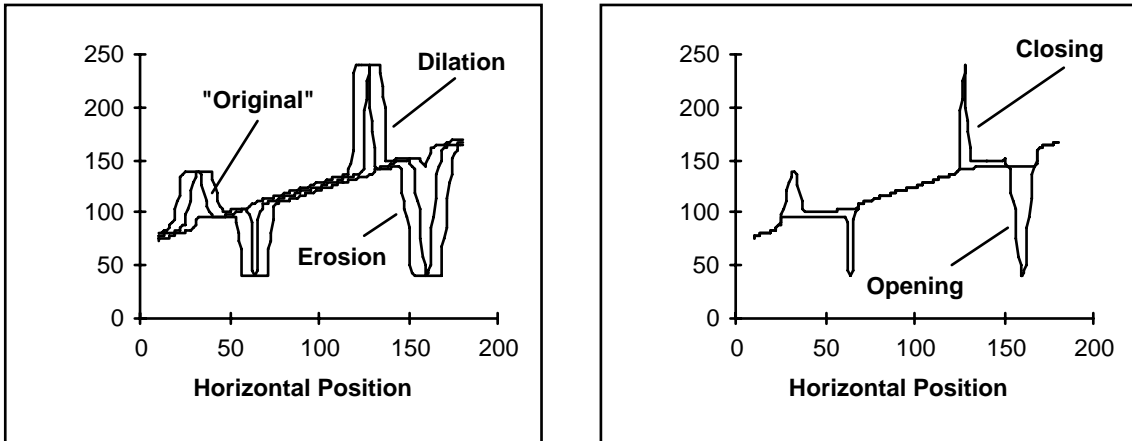
a) Effect of 15 \times 1 dilation and erosion b) Effect of 15 \times 1 opening and closing
