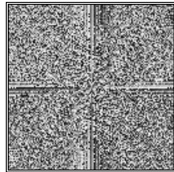
Figure 4c \varphi(\Omega,\Psi)
