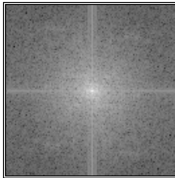
Figure 4b \log(|A(\Omega,\Psi)|)
